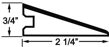
Reducer
