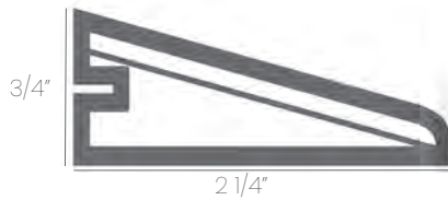
T-MOLD FOR PIONEERED® SOLID, NORTHERN SOLID SAWN® AND SOLID SAWN® STRUCTURED FLOORS
