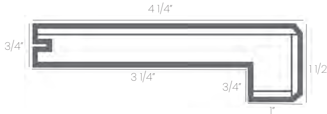
REDUCER FOR PIONEERED® SOLID, NORTHERN SOLID SAWN® AND SOLID SAWN® STRUCTURED FLOORS
